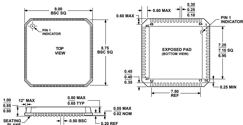
Figure 78. 64-Lead Lead Frame Chip Scale Package [LFCSP_VQ] 9 mm x 9 mm Body, Very Thin Octal (CP-64-3) Dimensions shown in millimeters
