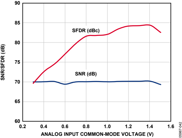
Figure 40. SNR/SFDR vs. Common-Mode Voltage, f_{IN} = 35\text{ MHz} , AD9222-50
