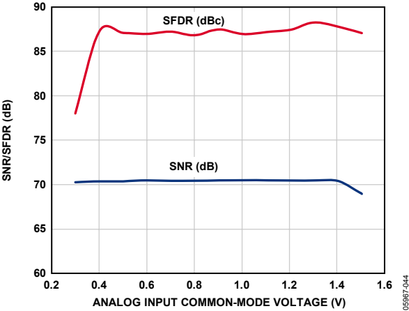
Figure 39. SNR/SFDR vs. Common-Mode Voltage, f_{IN} = 2.3\text{ MHz} , AD9222-50
