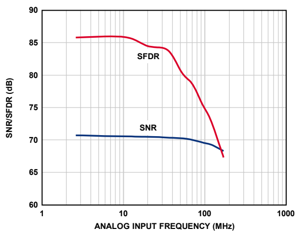
Figure 29. SNR/SFDR vs. f_{IN} , AD9222-50
