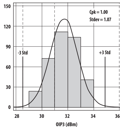
Figure 3. OIP3 @ 2 GHz, 4V, 60 mA. LSL = 28.5, Nominal = 31.0, USL = 36.0
