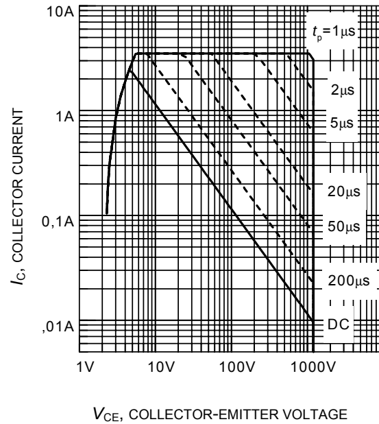
Figure 2. Safe operating area
