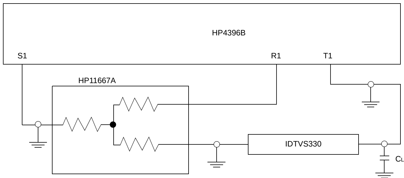
Figure 2. Gain/Phase, Crosstalk, Off-Isolation
