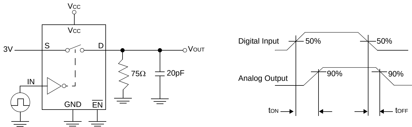
Figure 1. Switching Time
