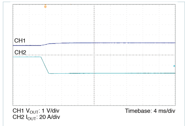
Figure 7 — 100% to 10% load transient response, V_{IN} = 28\text{ V} , nominal trim, C_{OUT\_EXT} = 1000\text{ }\mu\text{F}
