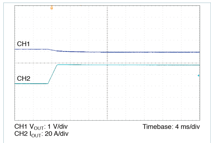
Figure 8 — 10% to 100% load transient response, V_{IN} = 28\text{ V} , nominal trim, C_{OUT\_EXT} = 1000\text{ }\mu\text{F}
