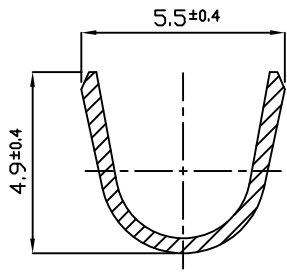
SECT. C-C SCALE : 5/1
