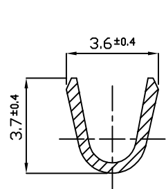
SECT. B-B SCALE : 5/1
