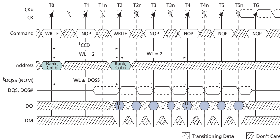
Figure 57: Consecutive WRITE-to-WRITE
