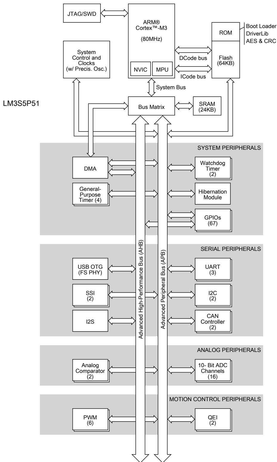
Figure 1-1. Stellaris LM3S5P51 Microcontroller High-Level Block Diagram
