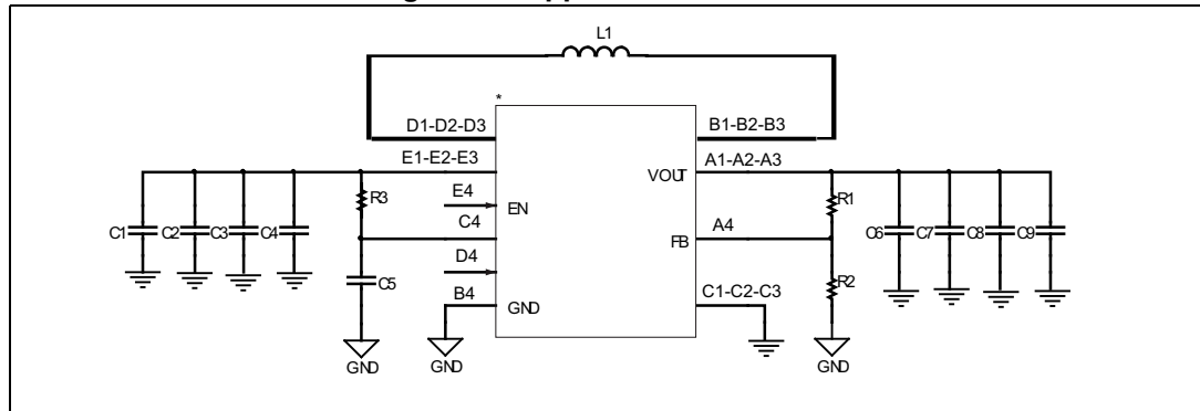
Figure 30. Application schematic
