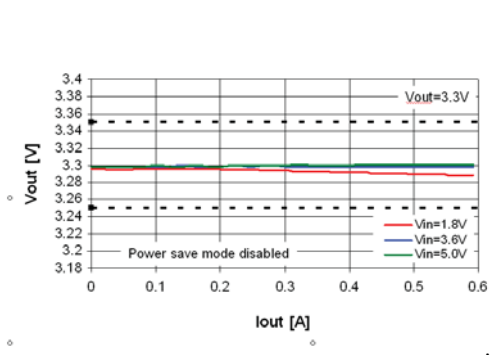
Figure 24. Output voltage vs. output current
