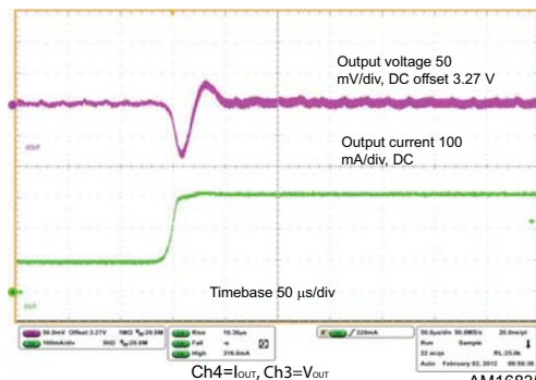
Figure 15. Load transient response @ V_{IN}=1.8\text{ V} , I_{OUT} = 100\text{ mA} to 300\text{ mA}
