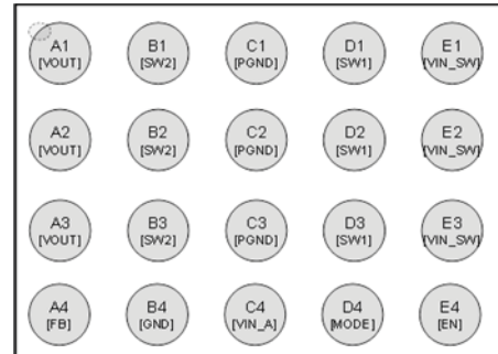
Figure 4. Pin connection bottom view
