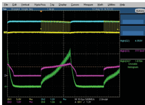
Figure 25. OCP threshold
