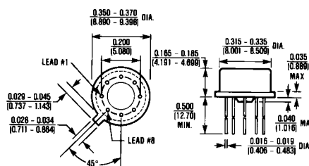
8 Lead TO-99 \theta_{JA} = 150^{\circ}\text{C/W} \theta_{JC} = 45^{\circ}\text{C/W}
