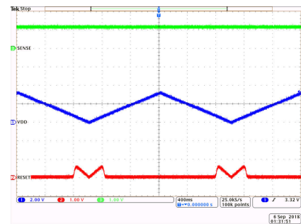
Figure 9-13. TPS3703-Q1 CT Bias Unlatch Function
