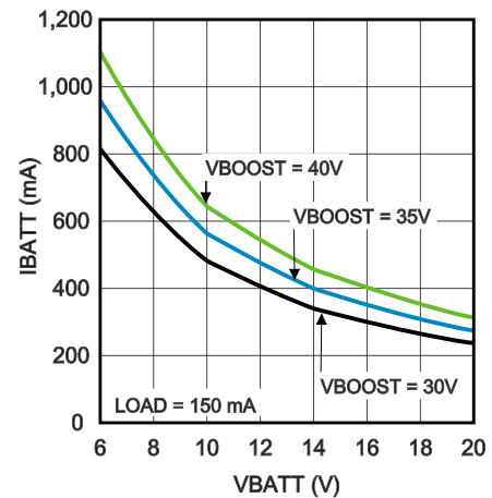
Battery Current
