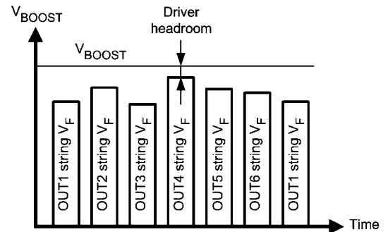
Boost Adaptive Control Principle with PSPWM 30138141
