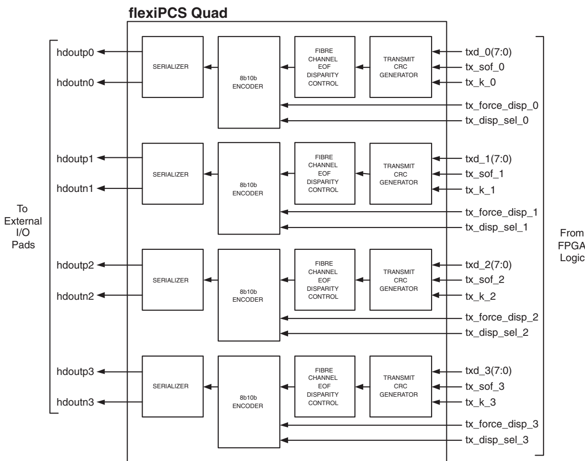
Figure 6-5. Fibre Channel Transmit Path (1 Quad)
