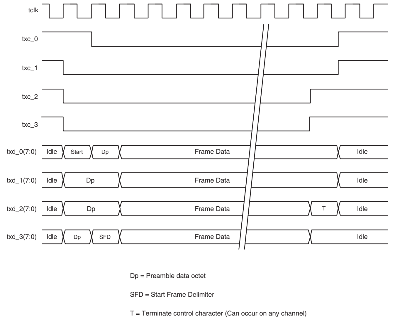
Figure 7-4. XAUI Transmit XGMII Interface Signals
