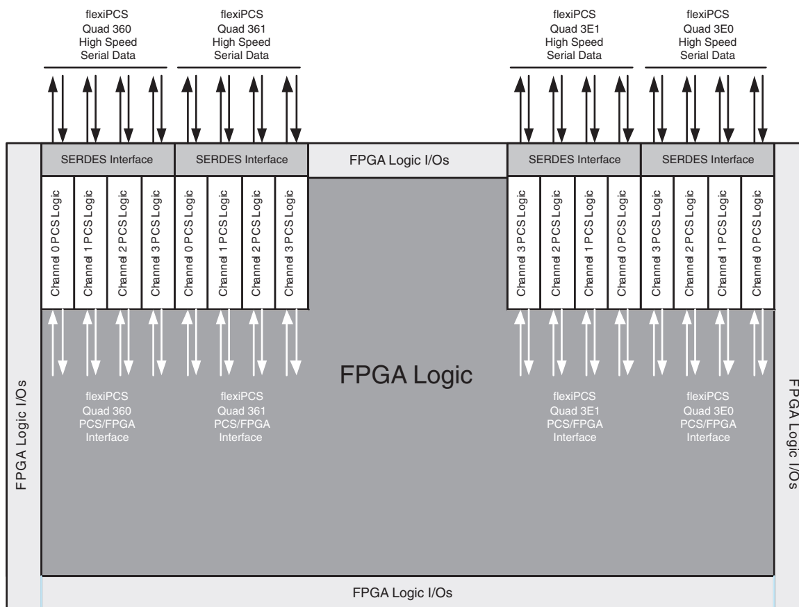
Figure 1-2. Example of LatticeSC Device with four flexiPCS Quads
