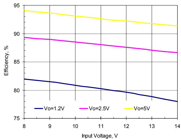
Figure 4. Efficiency vs. Input Voltage. Iout=5A
