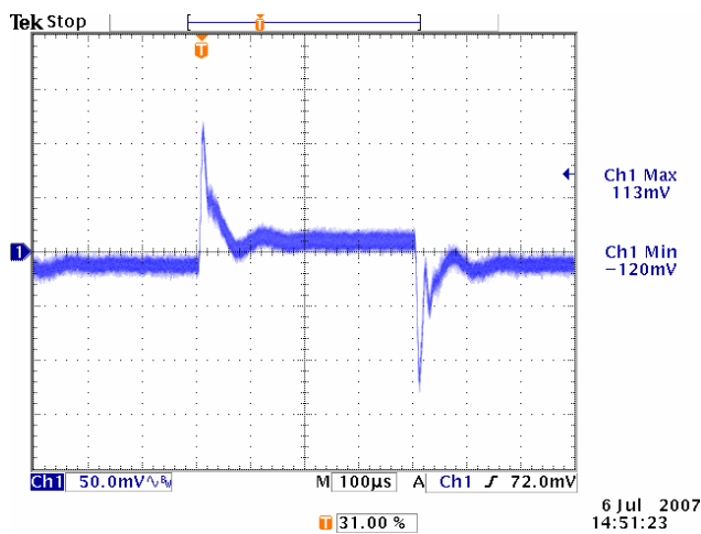
Figure 8. Vin=12V, Vout=5V. CCA=1
