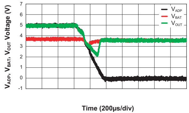
Response of Out when Switching from V_{ADP} to V_{BAT} ( V_{ADP} = 5V \rightarrow 0V ; V_{BAT} = 3.6V ; V_{ENBAT} = 5V ; V_{ENO} = 5V ; R_{LOAD} = 50\Omega )
