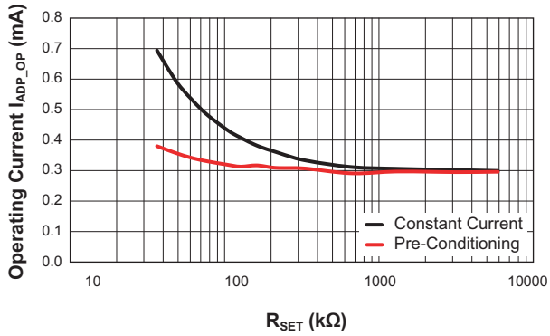
Adapter Supply Operating Current vs. R_{SET}
