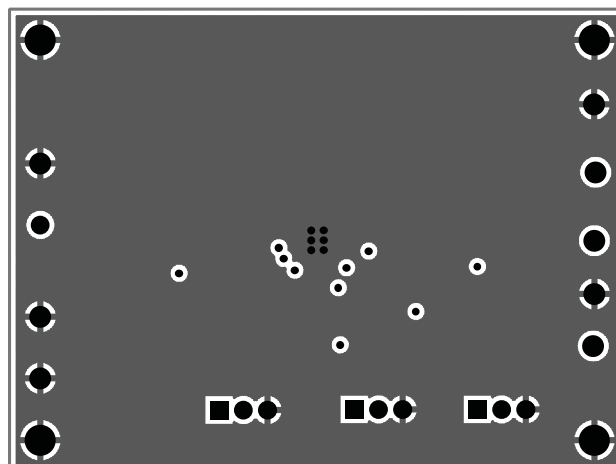
Figure 5: AAT3672-1/-2 Evaluation Board Mid1 Layer.
