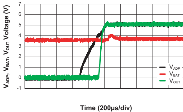
Response of Out when Switching from V_{BAT} to V_{ADP} ( V_{ADP} = 0V \rightarrow 5V ; V_{BAT} = 3.6V ; V_{ENBAT} = 0V ; V_{ENO} = 5V ; R_{LOAD} = 50\Omega )
