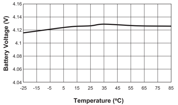
Recharge Voltage Threshold vs. Temperature ( V_{ADP} = 5V ; R_{SET} = 56.7k\Omega )
