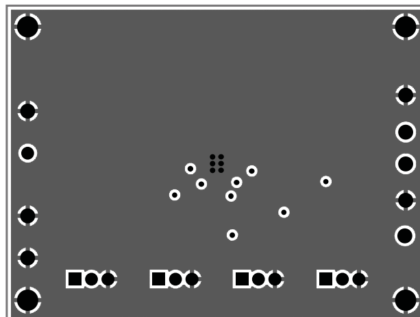
Figure 9: AAT3672-3 Evaluation Board Mid1 Layer.
