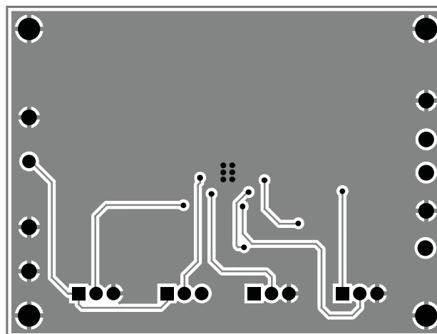
Figure 11: AAT3672-3 Evaluation Board Bottom Layer.
