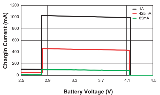
Constant Charge Current vs. Battery Voltage
