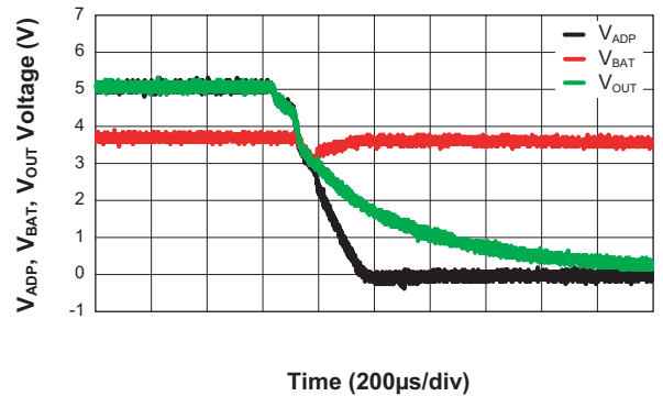
Response of Out when Switching from V_{ADP} to V_{BAT} ( V_{ADP} = 5V \rightarrow 0V ; V_{BAT} = 3.6V ; V_{ENBAT} = 0V ; V_{ENO} = 5V ; R_{LOAD} = 50\Omega )
