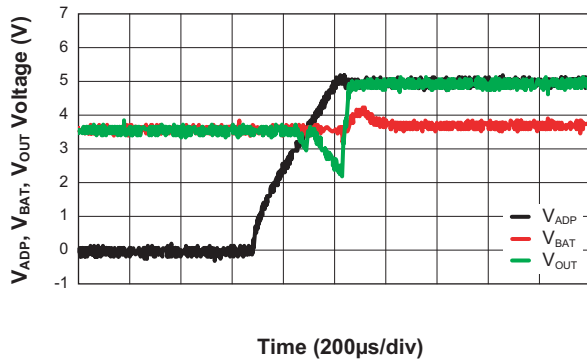
Response of Out when Switching from V_{BAT} to V_{ADP} ( V_{ADP} = 0V \rightarrow 5V ; V_{BAT} = 3.6V ; R_{LOAD} = 50\Omega )
