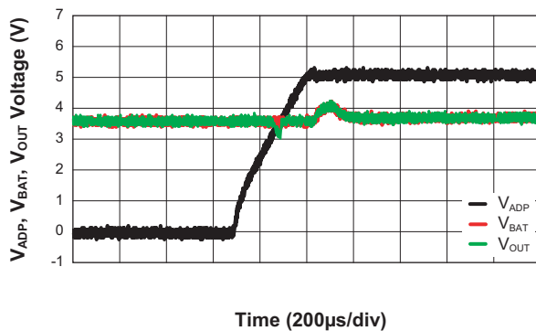
Response of Out when V_{ENO} = 0V ( V_{ADP} = 0V \rightarrow 5V ; V_{BAT} = 3.6V ; V_{ENBAT} = 5V ; R_{LOAD} = 50\Omega )
