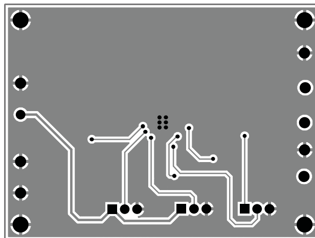
Figure 7: AAT3672-1/-2 Evaluation Board Bottom Layer.
