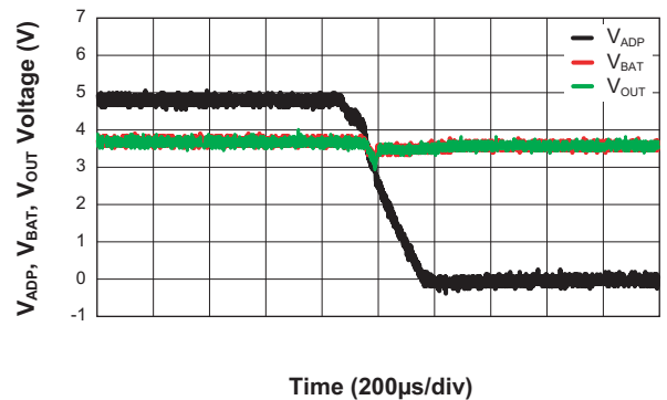
Response of Out when V_{ENO} = 0V ( V_{ADP} = 5V \rightarrow 0V ; V_{BAT} = 3.6V ; V_{ENBAT} = 5V ; R_{LOAD} = 50\Omega )
