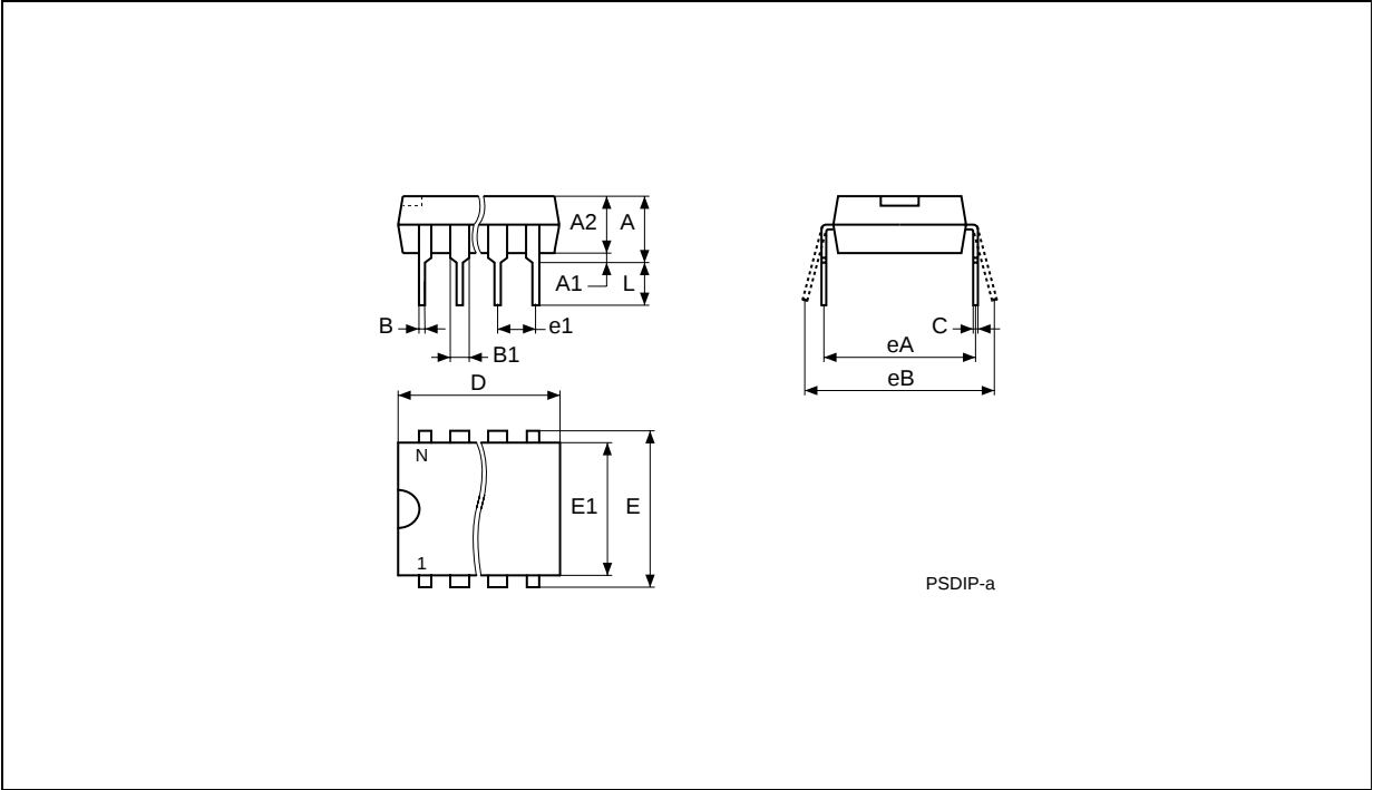
Figure 16. PSDIP8 (BN)
