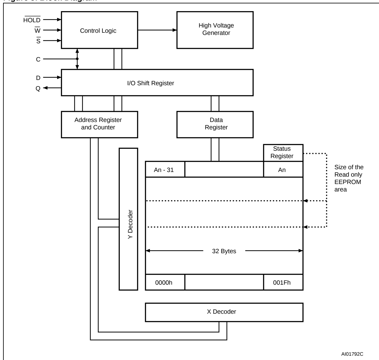
Figure 5. Block Diagram
