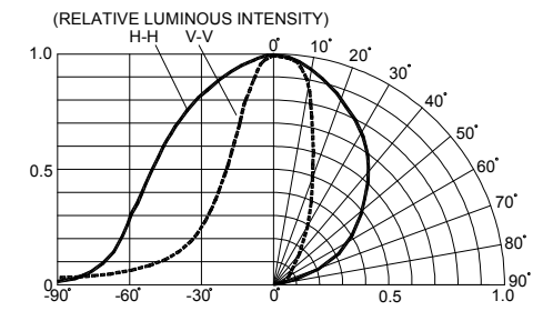
FIG.6 RED & BLUE&GREEN FAR FIELD PATTERN
