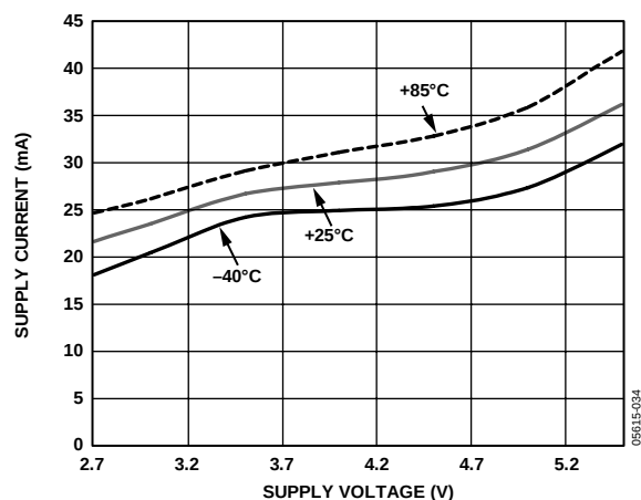
Figure 34. Current vs. VPOS
