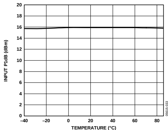
Figure 33. Input Compression vs. Temperature
