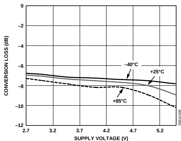
Figure 35. Conversion Loss vs. VPOS
