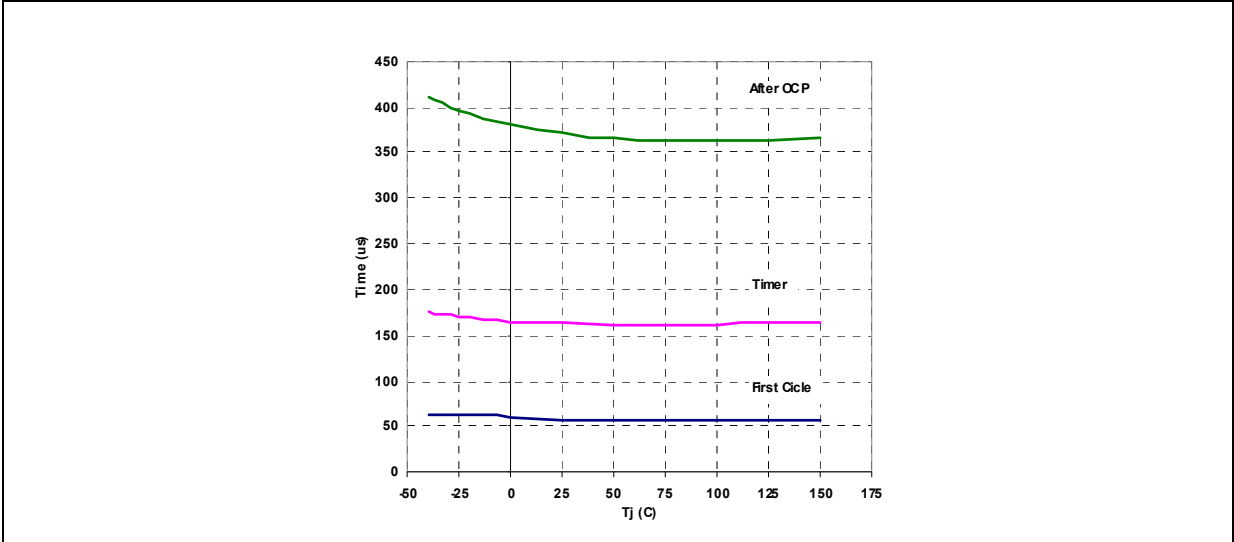
Figure 26. Start-up timer period vs. T_J
