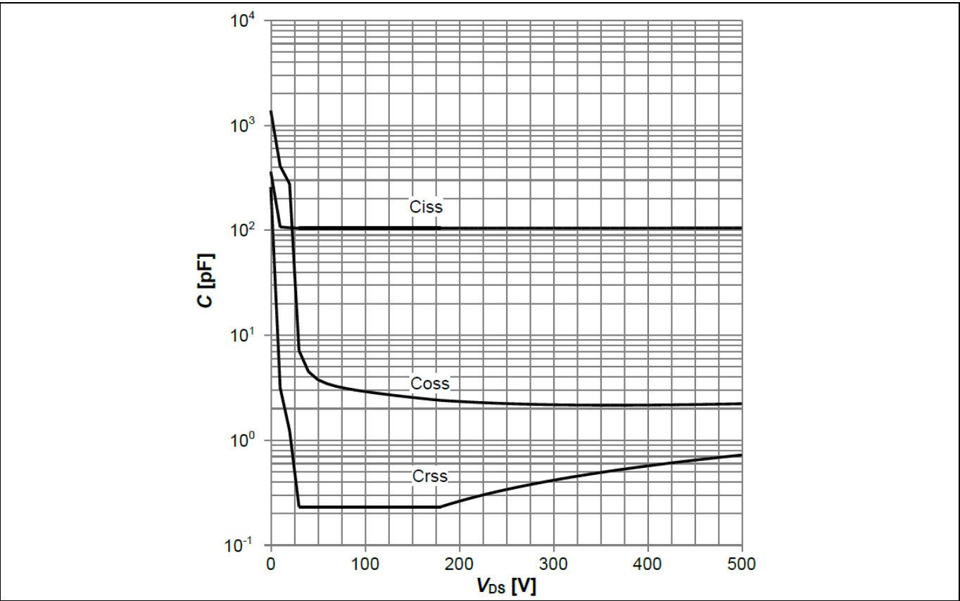
Figure 26 Typical CoolMOS™ capacitances of ICE5AR4780BZS ( C=f(V_{DS}); V_{GS}=0\text{ V}; f=250\text{ kHz} )
