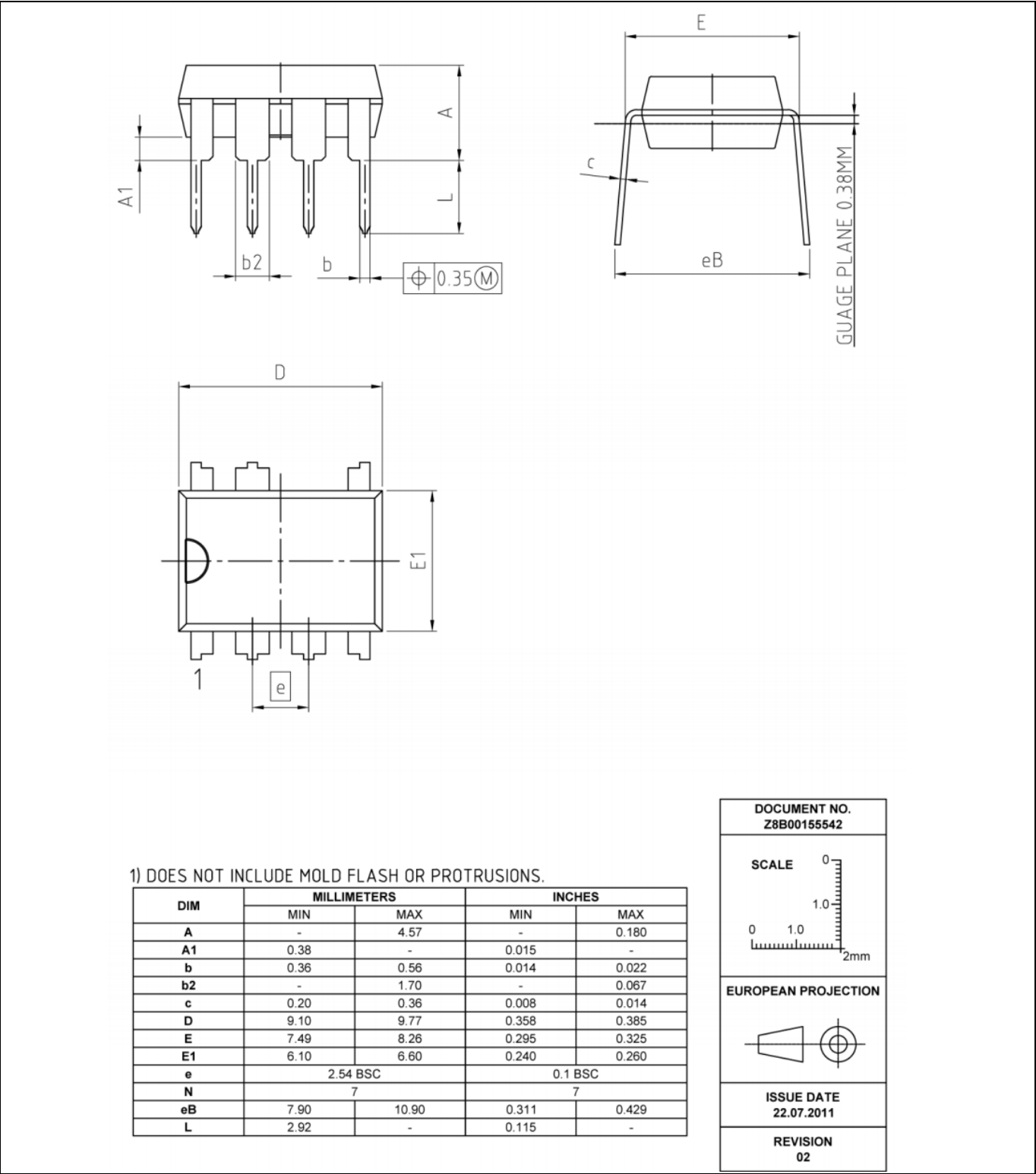
Figure 31 PG-DIP-7
