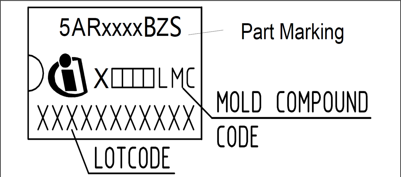
Figure 32 Marking of PG-DIP-7
