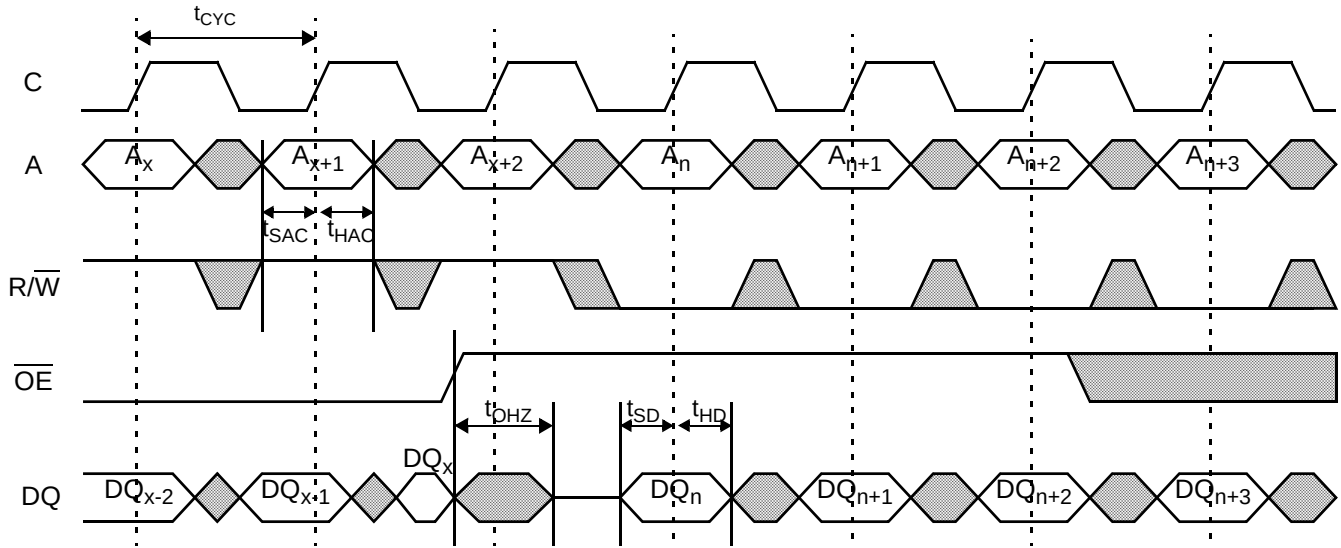
Figure 27. READ-to-WRITE for Pipelined Mode ( \overline{\text{OE}} Controlled) [41, 42]
