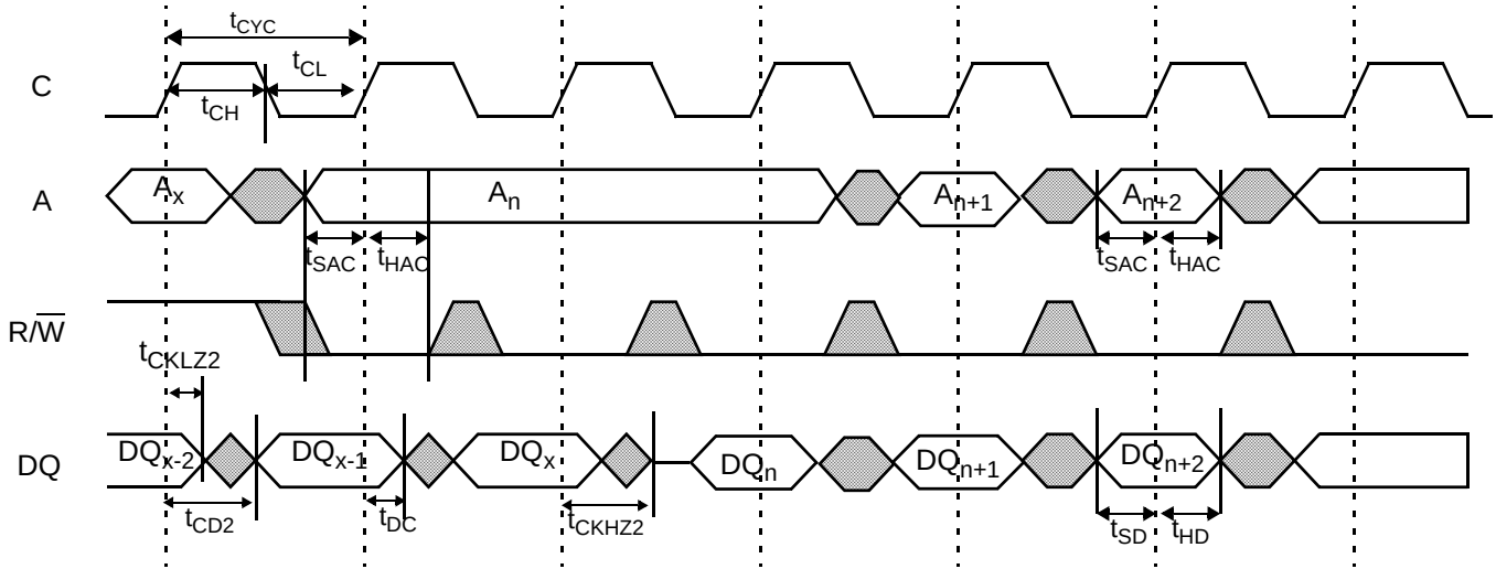
Figure 27. READ-to-WRITE for Pipelined Mode ( \overline{\text{OE}} Controlled) [41, 42]
