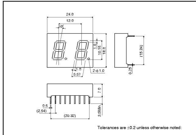
●External dimensions (Units : mm)
