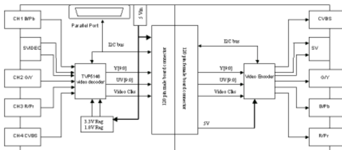
Figure 1–3. TVP5146EVM
