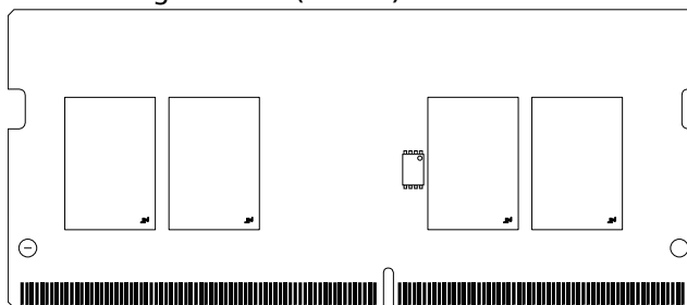
Figure 1: 260-Pin SODIMM (MO-310 R/C-A1)
