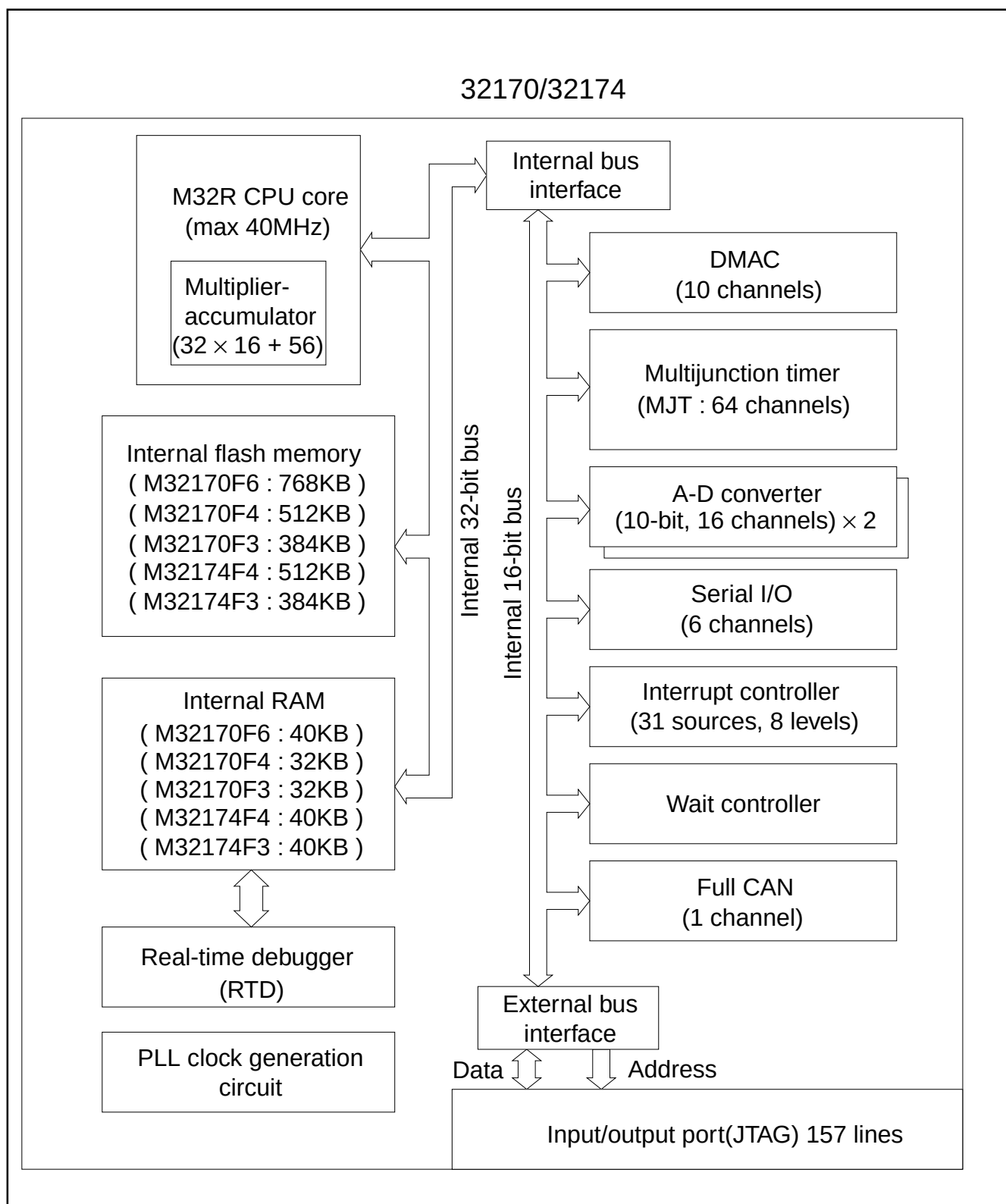
Figure 3 Block diagram
