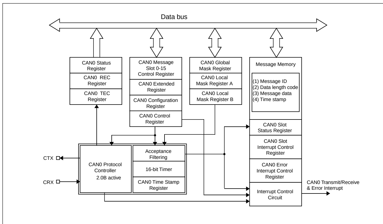
Figure 28 Block Diagram of the CAN Module
