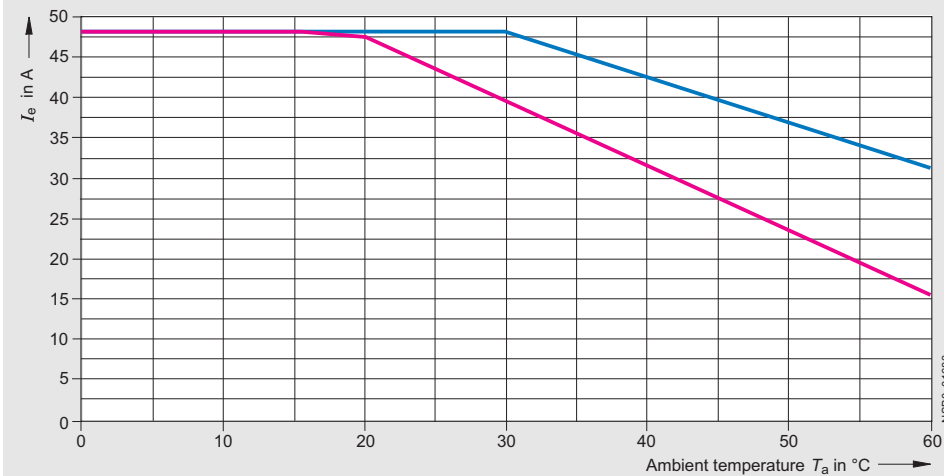
Type current 40 A (3RF24 40-AC..) 1)
