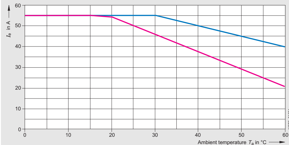
Type current 50 A (3RF24 50-AC..) 1)
