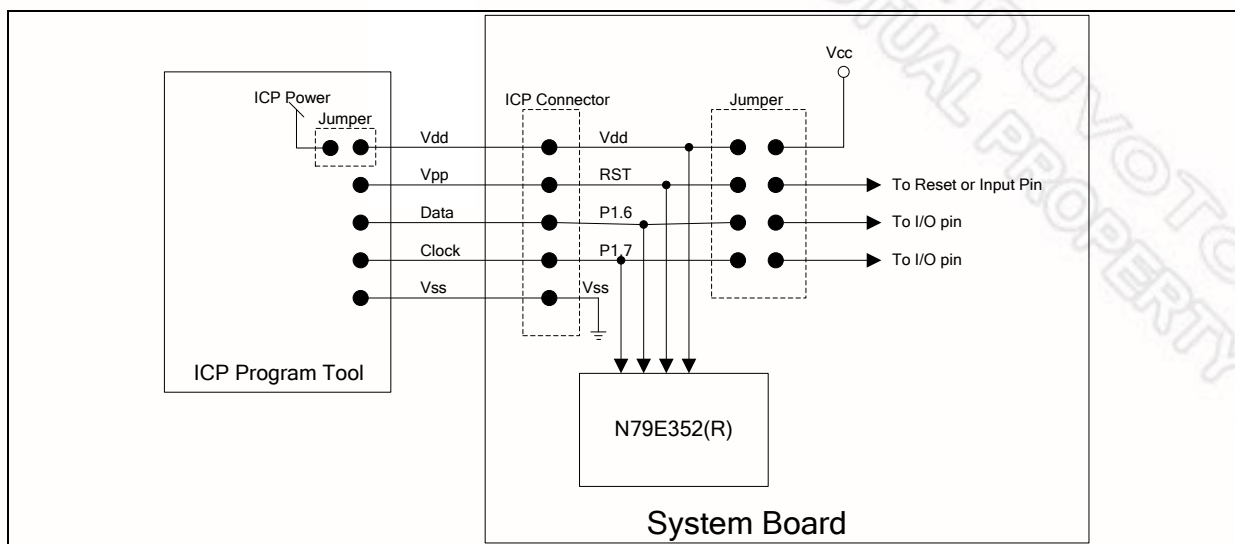
Figure 26-1: ICP Writer Tool connector pin assign
