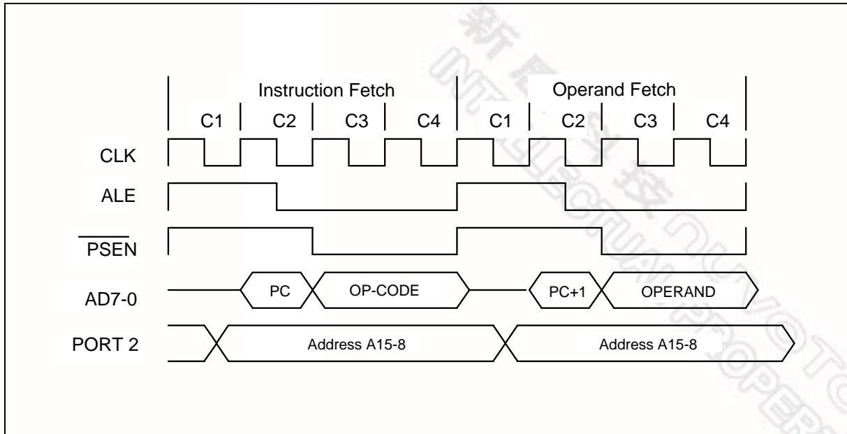
Figure 9-2: Two Cycle Instruction Timing
