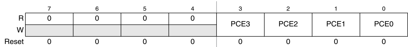
Figure 18-5. PIT Channel Enable Register (PITCE)
