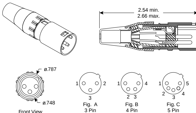
Dimensions (In.)
