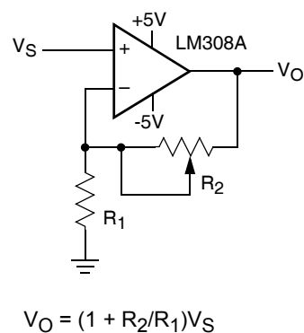
Noninverting Amplifier
