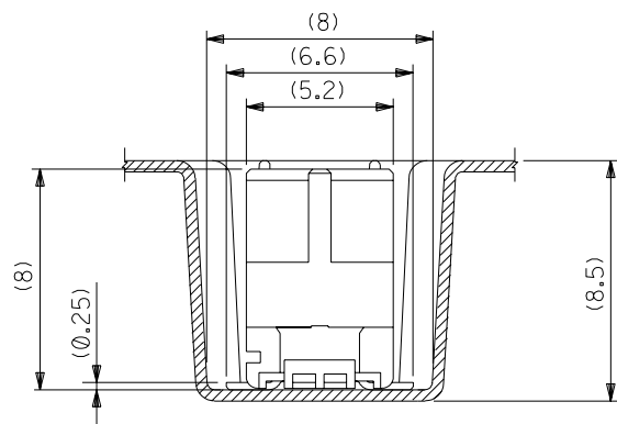
SECT. X-X
