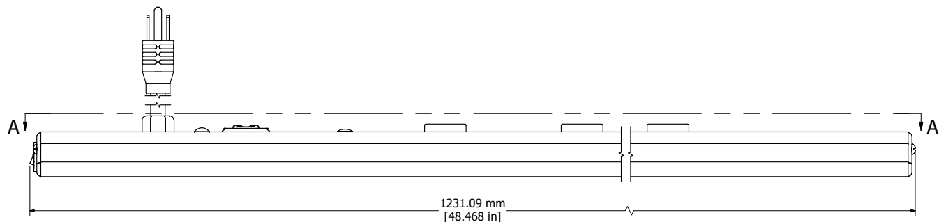
ASSEMBLY - VIEW FROM SIDE
