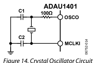
Figure 14. Crystal Oscillator Circuit
