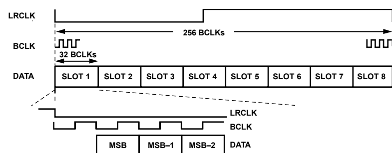
Figure 34. TDM Mode
