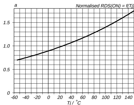
Fig.9. Normalised drain-source on-state resistance. a = R_{DS(ON)} / R_{DS(ON)25^\circ \text{C}} = f(T_J) ; I_D = 3.2 \text{ A} ; V_{GS} = 10 \text{ V}
