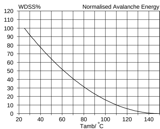
Fig.15. Normalised avalanche energy rating. W_{DSS}\% = f(T_{amb}) ; conditions: I_D = 3.2 A
