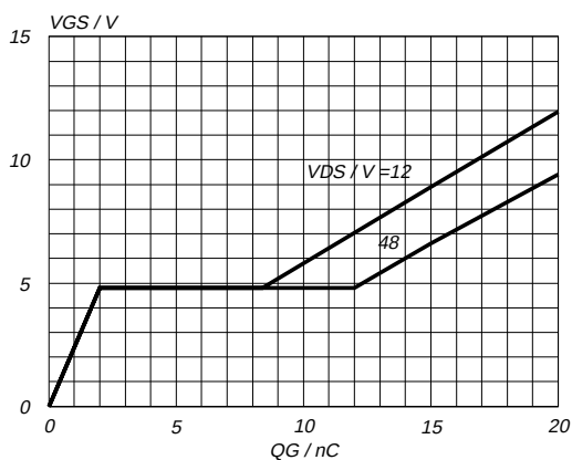
Fig.13. Typical turn-on gate-charge characteristics. V_{GS} = f(Q_G) ; conditions: I_D = 3.2 A; parameter V_{DS}
