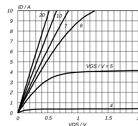
Fig.5. Typical output characteristics, T_j = 25^\circ\text{C} . I_D = f(V_{\text{DS}}) ; parameter V_{\text{GS}}
