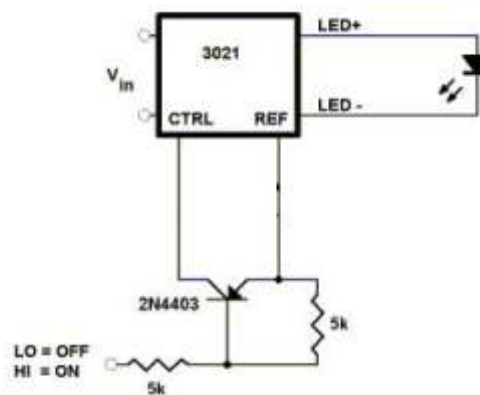
Figure 14. Pulse/Strobe input 5V=ON
