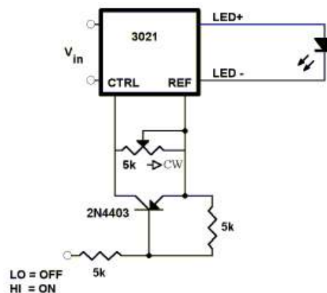
Figure 12. External dimming plus ON/OFF control with logic level input
