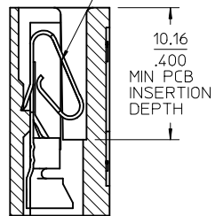
SECTION Z-Z
