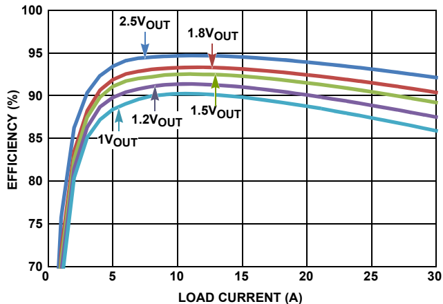
FIGURE 6. EFFICIENCY vs LOAD CURRENT (PARALLEL SINGLE OUTPUT, AS SHOWN IN Figure 19 AT 5V_{\text{IN}} /500kHz)
