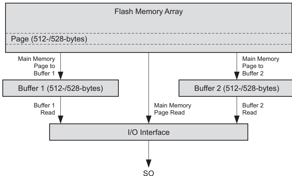
Figure 21-1. Block Diagram
