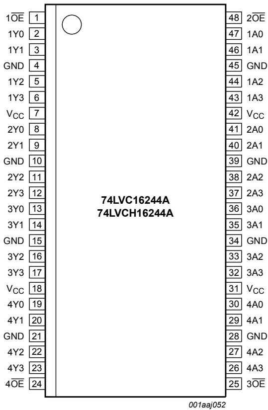
Figure 4. Pin configuration SOT370-1 (SSOP48) and SOT362-1 (TSSOP48)
