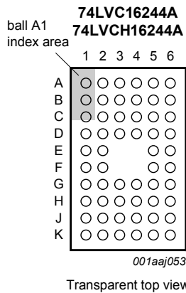
Figure 5. Pin configuration SOT702-1 (VFBGA56)
