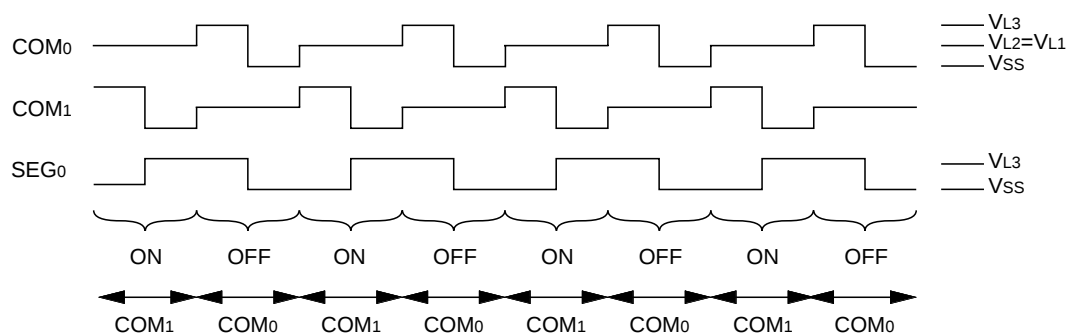
Fig. 46 LCD drive waveform (1/2 bias)
