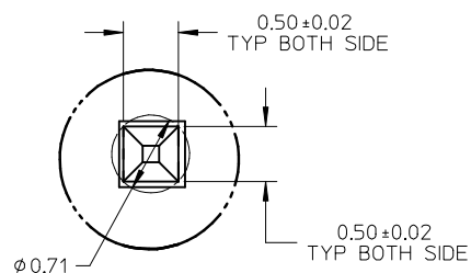
DETAIL Z
