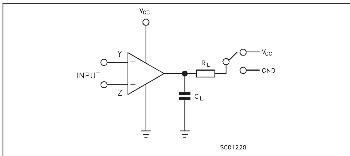
Figure 2 : Propagation Delays
