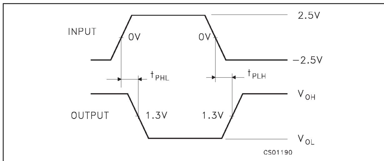
Figure 2 : Propagation Delays
