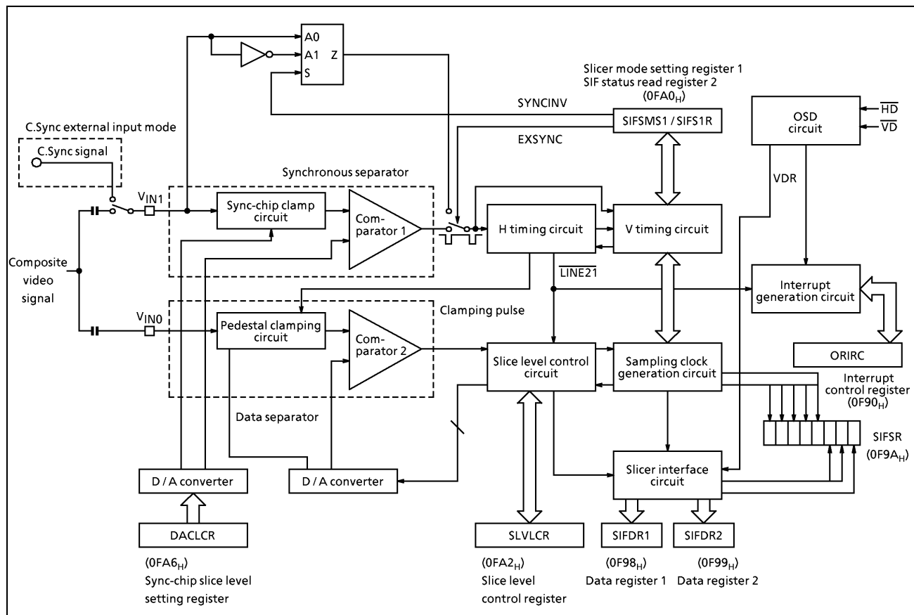
Figure 2-86. Data Slicer
