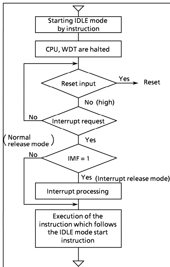
Figure 1-18. IDLE Mode
