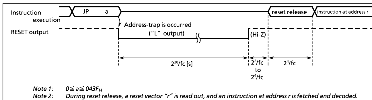
Figure 1-29. Address-Trap-Reset
