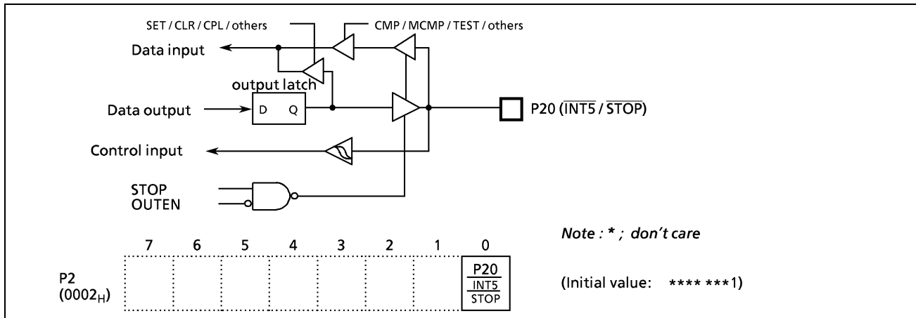
Figure 2-3. Port P2
