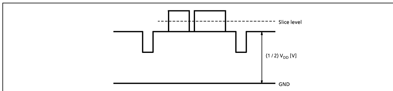
Figure 2-91. Pedestal Clamp
