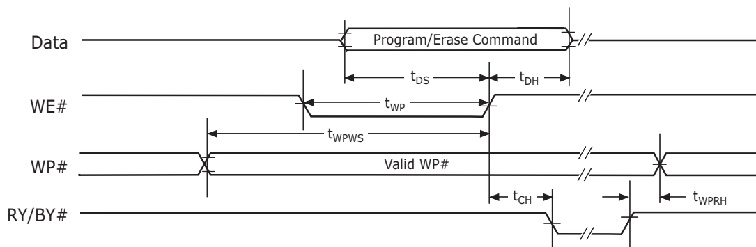
Figure 20. WP# Timing
