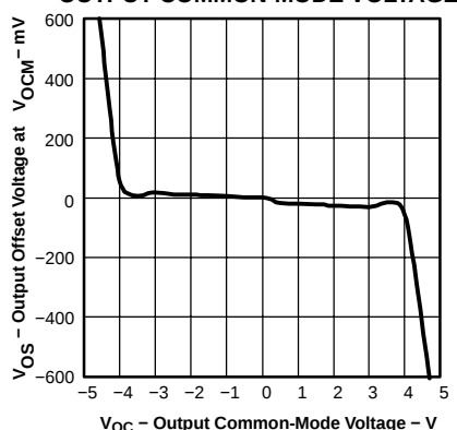
OUTPUT OFFSET VOLTAGE AT V_{OCM} vs OUTPUT COMMON-MODE VOLTAGE
