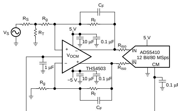
Using the THS4503 With the ADS5410 Figure 97
