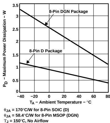
Figure 113. Maximum Power Dissipation vs Ambient Temperature
