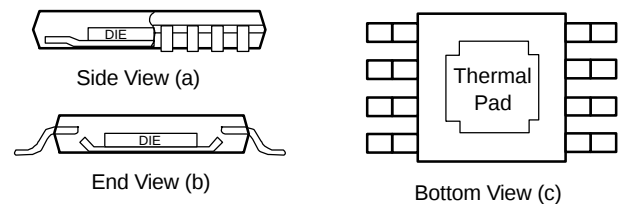
Figure 111. Views of Thermally Enhanced Package
