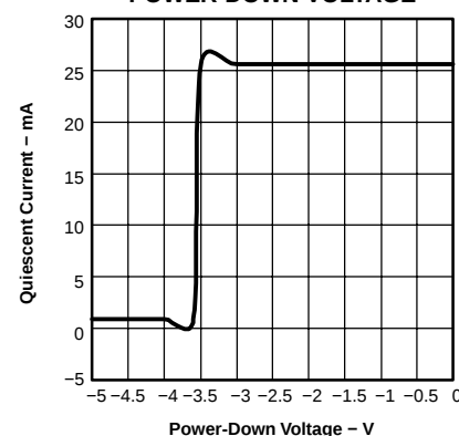
QUIESCENT CURRENT vs POWER-DOWN VOLTAGE
