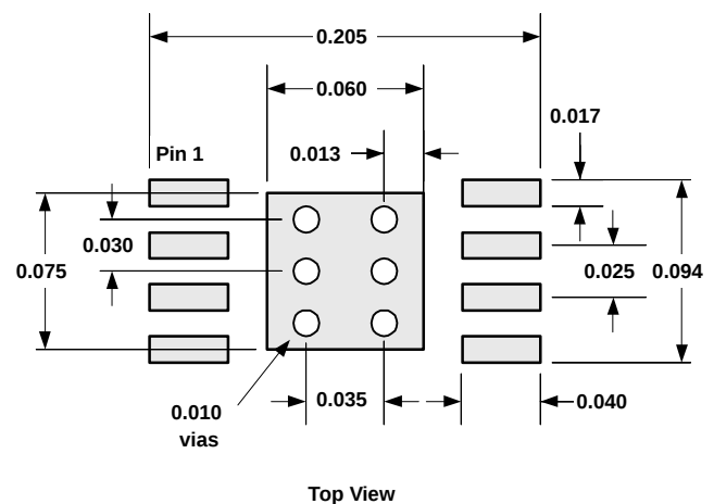
Figure 112. PowerPAD PCB Etch and Via Pattern
