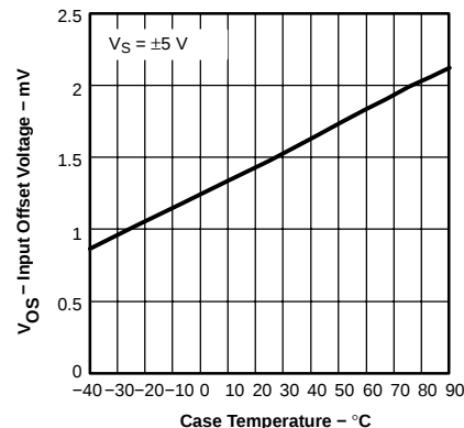
INPUT OFFSET VOLTAGE vs CASE TEMPERATURE
