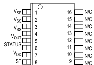
Figure 2. Pin Connections
