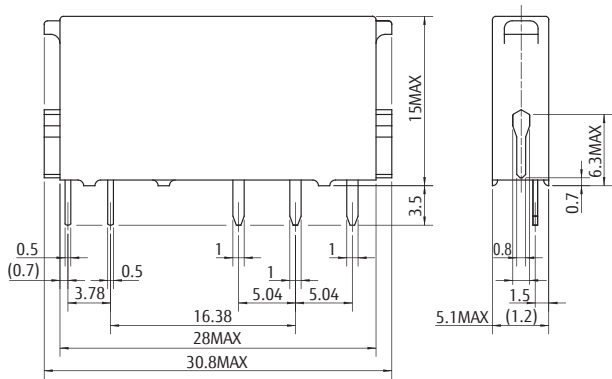
Socket type
