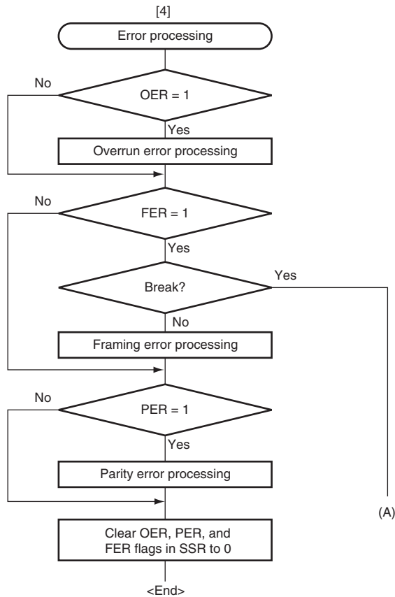
Figure 14.8 Sample Serial Reception Data Flowchart (2)
