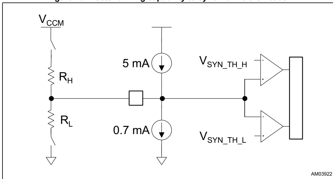
Figure 40. Master driving capability to synchronize the L6985F
