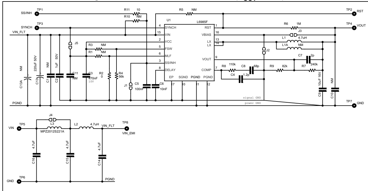
Figure 41. Evaluation board schematic ( V_{OUT} = 3.3\text{ V} )
