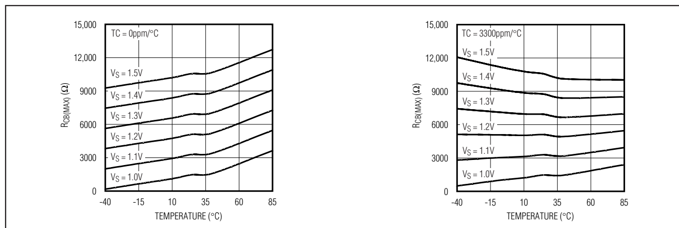
Figure 10. Adjustable Turn-On Voltage
